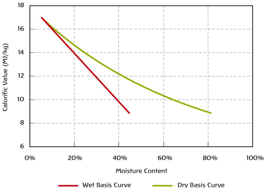
Figure A2.1 ● Calorific Values of Fuelwood
